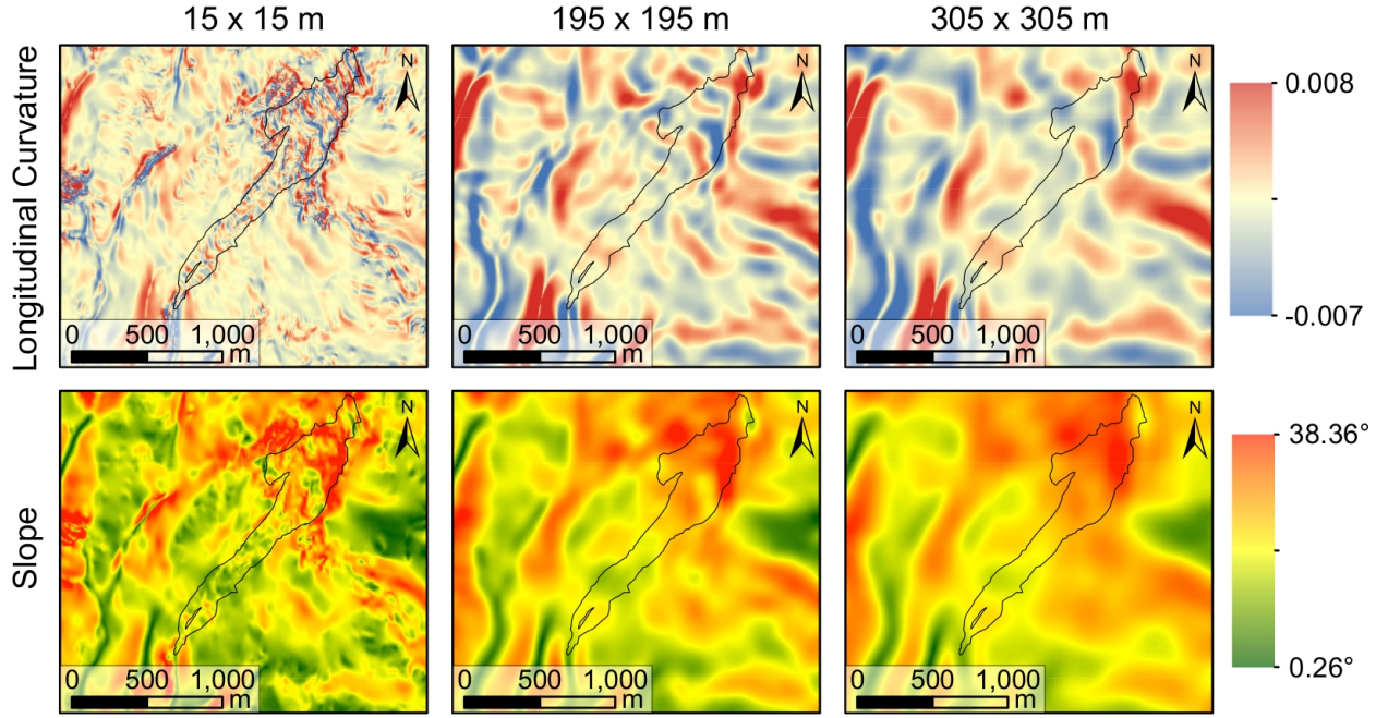
Figure 7: Illustration of the multiscale resampling approach of the DTM used on the LA VALETTE dataset. This figure shows the influence of the window size parameter \varrho on the computation of the slope and curvature of the terrain.
