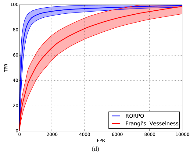
Figure 4: The initial image and the ground truth (a), the result of the RORPO multiscale (b) and the result of the Frangi's Vesselness (c). The mean and standard deviation of the ROC curves (d).
