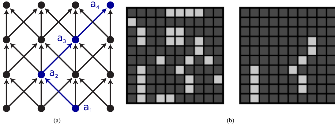
Figure 1: (a) A graph G (in black) defining a global vertical path orientation and a path (in blue) of length 4 pixels. (b) An example of a path opening of length 4 pixels. From left to right, the initial image and the result of the path opening. Only pixels belonging to a path of at least 4 pixels are kept. Paths are defined using the graph of figure (a).
