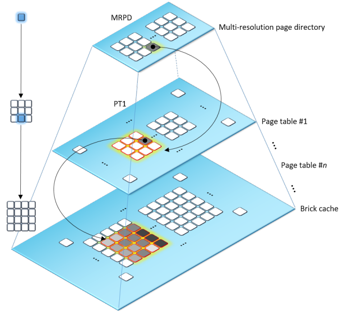
Fig. 2. Multi-resolution, multi-level page table hierarchy virtualization principle. A 2D representation of our 3D addressing structure. In this example, only one intermediate level of virtualization is used (PT1). One entry of the MRPD addresses a PT block of 3 \times 3 entries in the PT1 cache and one entry in the PT1 cache addresses a brick of 4 \times 4 voxels in the data cache.
