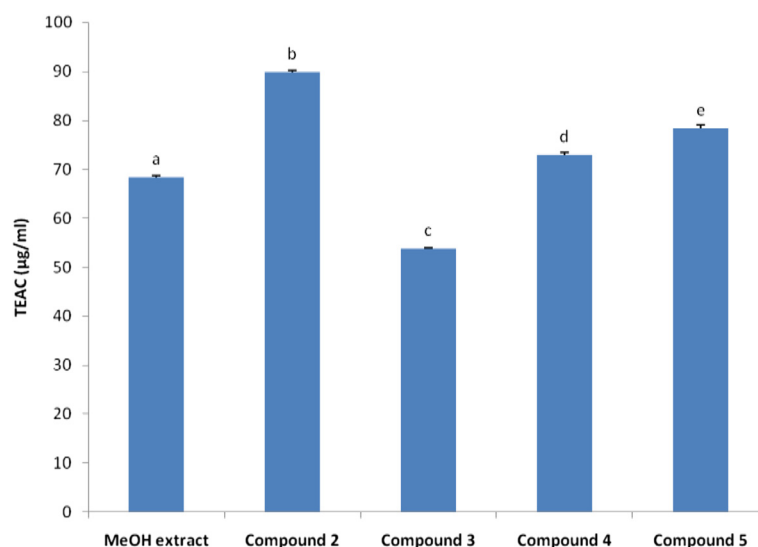
Figure 3 Gallic acid equivalent antioxidant capacity (TEAC; µg/ml) of tested samples. Bars represent the mean ± SD of three independent experiments carried out in triplicate. Letters a-e indicate significant differences between samples according to one way ANOVA and Waller Duncan test; p < 0.05 .
