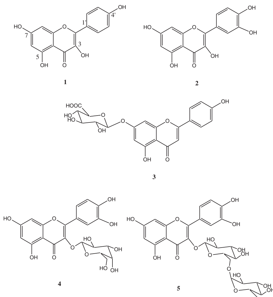
Figure 1 Chemical structures of the isolated compounds from O. spinosa . 1 : kaempferol; 2 : quercetin; 3 : apigenin-7-O- \beta -D-glucuronopyranoside; 4 : quercetin 3-O- \beta -D-galactopyranoside; 5 : quercetin 3-O- \alpha -L-rhamnopyranosyl (1 \rightarrow 6) \beta -D-glucopyranoside.
