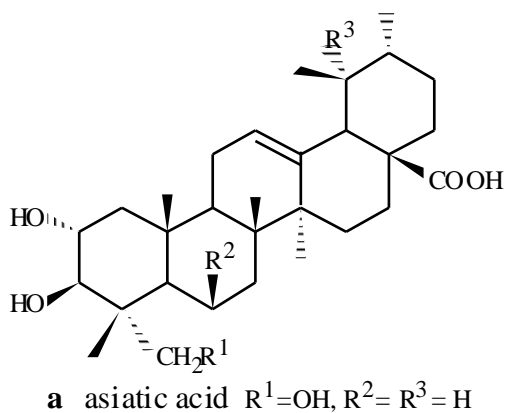
Fig. 1. Structures of genins of tested saponins.
