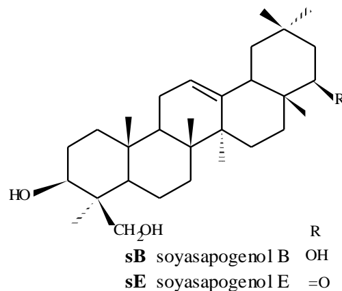
Fig. 1. Structures of genins of tested saponins.
