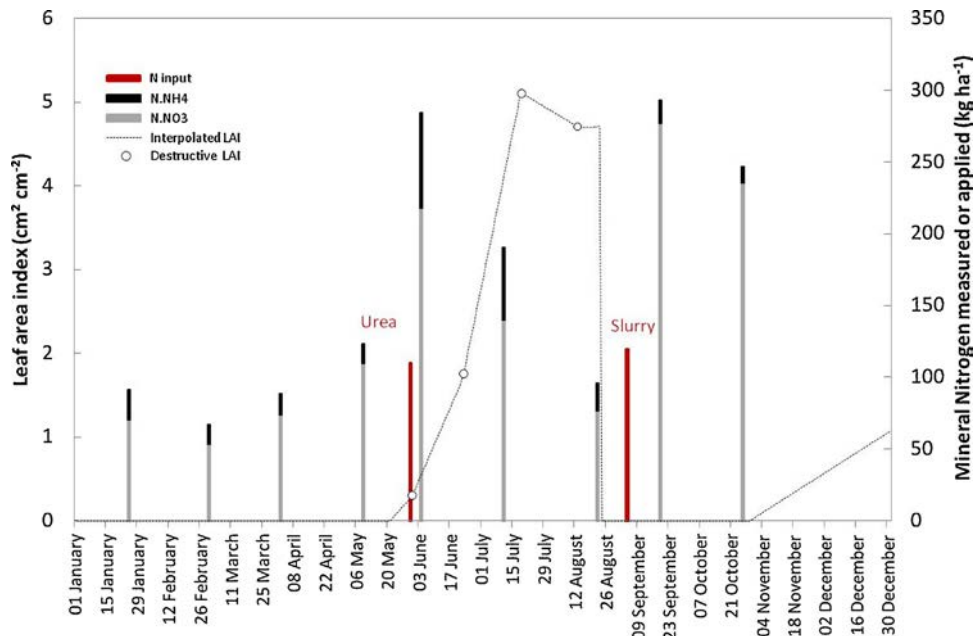
Fig. 6. Daily leaf area index dynamics of maize, soil mineral nitrogen content dynamics in the upper layer (0–30 cm, grey and black bars) and mineral nitrogen input (red bars) during 2012. (For interpretation of the references to color in this figure legend, the reader is referred to the web version of this article.)
