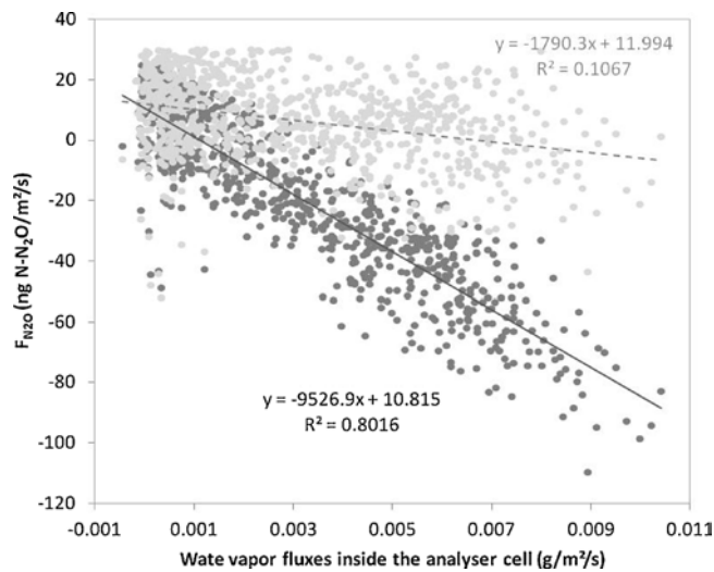
Fig. 11. Half-hourly \text{N}_2\text{O} fluxes versus water vapour fluxes from 1 July to 18 August 2012. Light grey circles: no density correction, dark grey circles: with only WPL correction applied. The solid lines indicate the results of least-squares linear regressions for both datasets.
