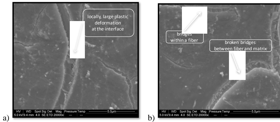
Figure 4 - SEM micrographs of epoxy composites reinforced with flax fabric modified with ELO (2.5 wt-%) and by EB-irradiation (20 kGy) after tensile testing in the 45° orientation until breakage: (a) plastic deformation on the interphase between 2 fibers, and (b) broken bridges between one fiber and the matrix, and in other zones, plastically deformed bridges within a fiber.
