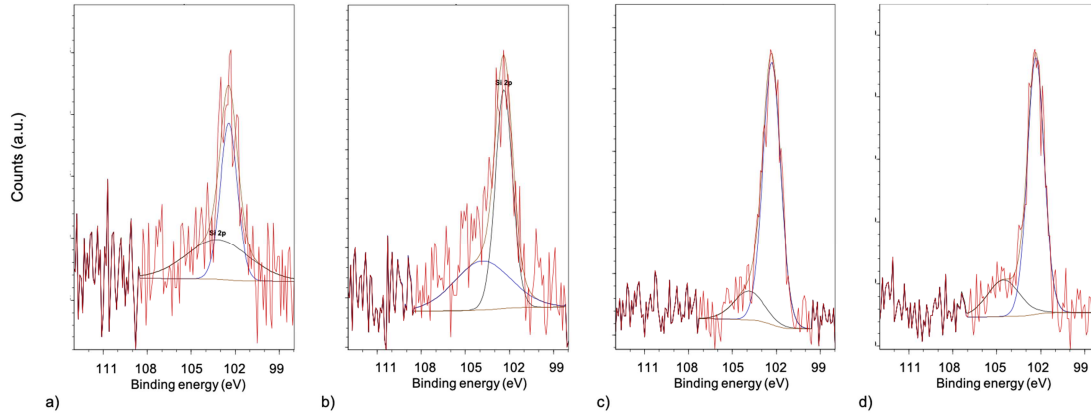
Figure 8 – High-resolution Si2p XPS spectra of FTA fibers, (a) in the unmodified state, (b) after peroxidation by 50 kGy EB irradiation, (c) after grafting of the vinyltrisiloxane by thermal reaction, and (d) after washing out of the ungrafted siloxane model compound.
