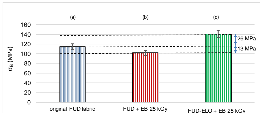
Figure 6 – Comparison of tensile strength for the 2-ply FUD-based epoxy composites measured in the main direction of the flax fibers: (a) original FUD fabric, (b) fabric after 25 kGy EB-treatment and (c) after sorption of ELO (2.5 wt-%) and subsequent EB-grafting at 25 kGy.
