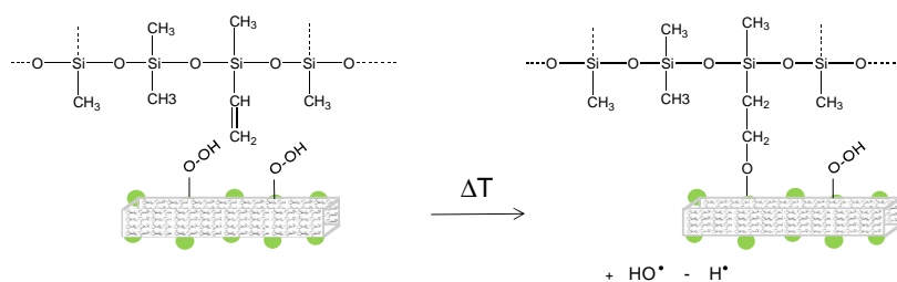
Scheme 3 – Sketch representing the grafting process based on the thermal activation of a peroxidized cellulosic substrate with a silicone matrix including vinylsiloxane units.
