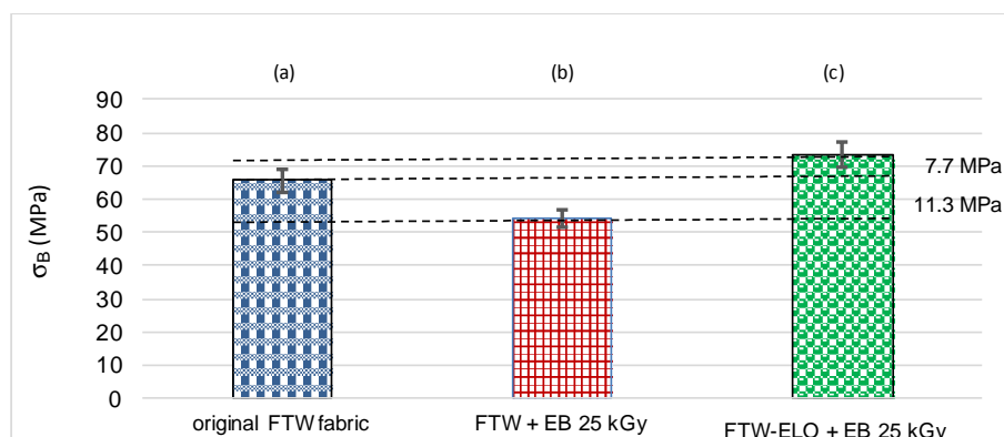
Figure 2 – Comparison of tensile strength for the 8-ply FTW-based epoxy composites measured in the 45° direction: (a) original fabric, (b) fabric after 25 kGy EB-treatment and (c) after sorption of ELO (2.5 wt-%) and subsequent EB-grafting at 25 kGy.
