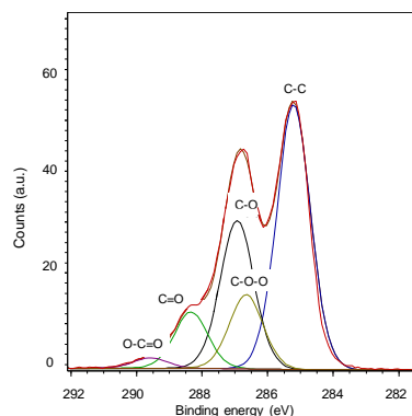
Figure 7 – High-resolution C1s XPS spectrum of FTA fibers after peroxidation by EB-irradiation at 50 kGy in air.
