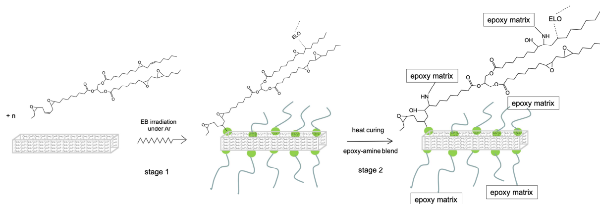
Scheme 2 – Sketch illustrating the principle of radiation-assisted attachment of epoxidized linseed oil onto natural fibers (stage 1), and the coupling between the matrix and the fibers through covalent linkages (stage 2).
