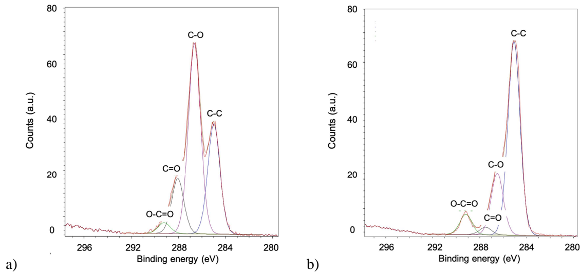
Figure 1 – High-resolution C1s XPS spectra of (a) acetone-washed flax fibers before treatment and (b) after sorption of ELO, EB-irradiation at 20 kGy and removal of ungrafted ELO (b).
