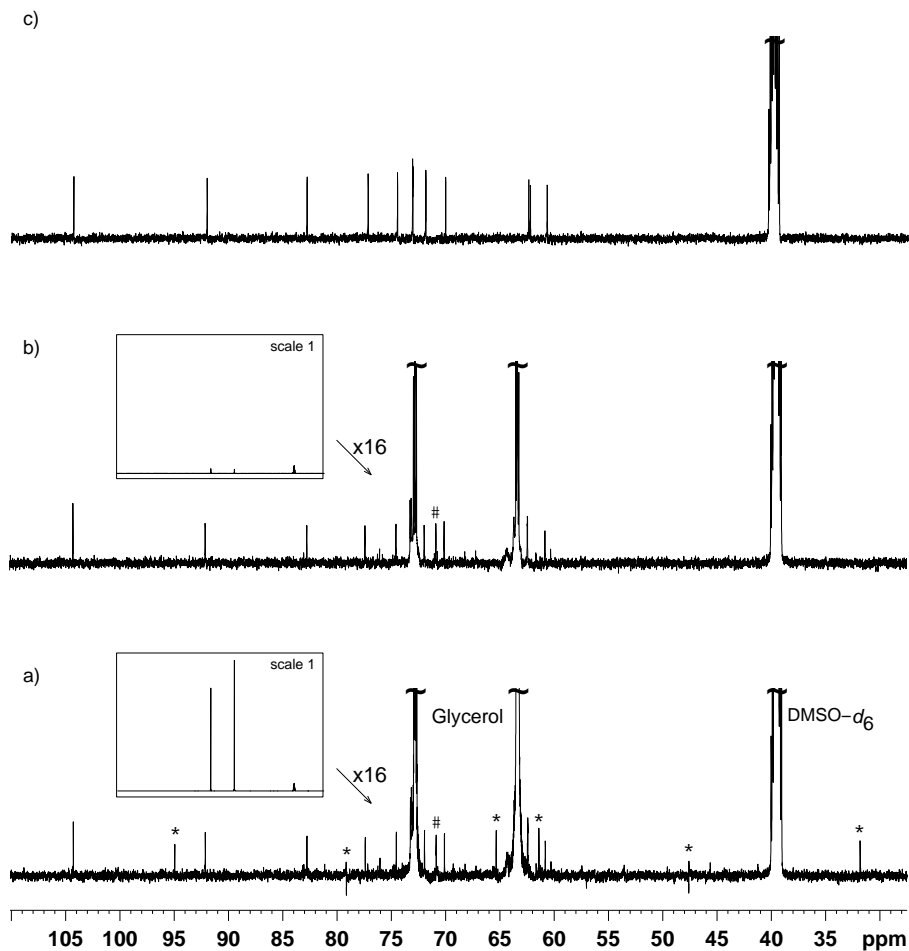
Figure 3. a) ^{13}\text{C} NMR spectrum of D(+)-sucrose (24 mM) and glycerol (3.6 M) in DMSO- d_6 . The "*" sign indicates decoupling artifacts. The "#" sign indicates a signal from a minor compound contained in bio-sourced glycerol; b) Analysis of the same sample as in a) but with multiple presaturation of glycerol signals. The framed inserts show spectra overviews drawn at full vertical scale. In spectrum a) the resonance peaks of DMSO- d_6 (the rightmost ones) are much smaller than those of glycerol while in b) the latter are hardly visible, thus demonstrating the efficiency of the glycerol resonance peak elimination. c) ^{13}\text{C} NMR spectrum of D(+)-sucrose (24 mM) in DMSO- d_6 . All acquisitions required the recording of 128 scans preceded by 8 dummy scans.
