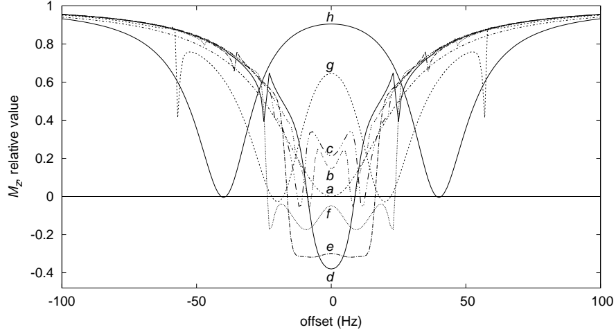
Figure 2. Saturation profiles for presaturation at two sites , at \pm\Omega^{\text{sat}}/2\pi for \Omega^{\text{sat}}/2\pi = 0, 2, 4, 6, 8, 10, 20, 40 Hz, corresponding to traces a to h . The relaxation times T_1 and T_2 are both equal to 0.5 s. The relaxation delay lasts 5 s during which 10 presaturation modules of 0.5 s each are applied. Each module is made of 50000 slices, for which \Omega_{1x} and \Omega_{1y} values are calculated with \Omega_1/2\pi = 50 Hz.
