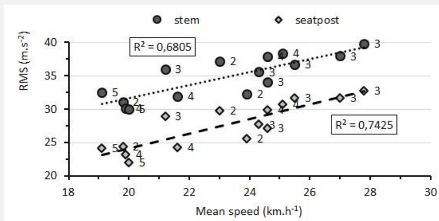
Figure 2. Linear relationship between RMS value and mean speed. Difficulty of each cobbles sector is indicated by the number to the right of the mark
