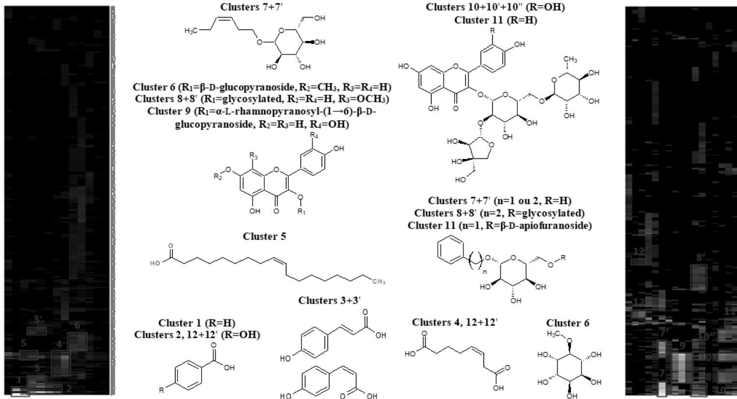
Figure 1. ^{13}\text{C} NMR chemical shift clusters obtained by applying HCA on EAF (left) and n -BFC (right) CPC fractions from C. arborescens .
