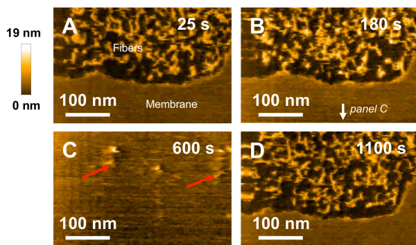
FIGURE 8 | Interaction between fibrillar WT peptides and a POPC/SM/Chol/GM1 membrane. Successive HS-AFM height images extracted from video 5 25 s after injection (A), 180 s after injection (B), 600 s after injection, and 1100 s after injection. Fibers present on the membrane are pointed by red arrows on (C).
