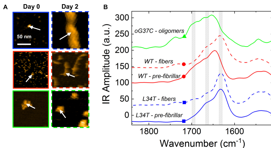
FIGURE 4 | Representative NanoIR spectra coming from \text{A}\beta_{1-42} peptide variants in early and late stages of aggregation. (A) Representative AFM images of isolated structures of the different \text{A}\beta_{1-42} peptides variants for pre-fibrillar or fibrillar species obtained after 0 or 2 days of fibrillation, respectively. (B) Associated representative NanoIR spectra, acquired locally on the isolated structures. The WT peptides are represented in red, L34T in blue, and oG37C in green. Gray bands centered at 1630, 1660 and 1690 \text{cm}^{-1} indicate, respectively, parallel \beta -sheet, \beta -turn, and anti-parallel \beta -sheet. White arrows on (A) represent the position of the NanoIR tip when acquiring NanoIR spectra.
