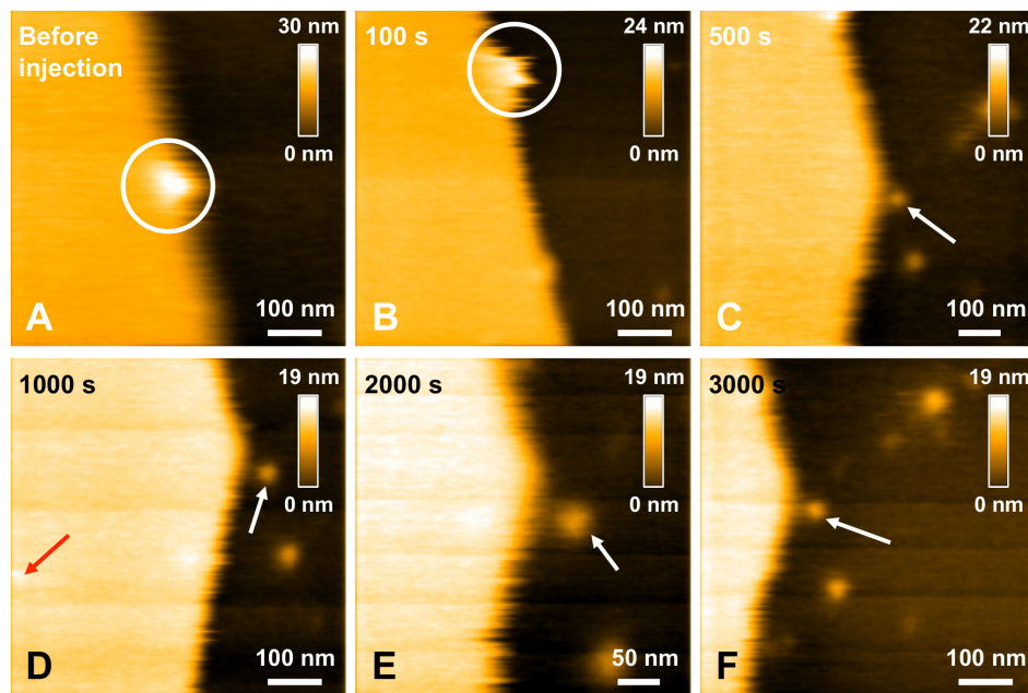
FIGURE 7 | Interaction between L34T mutant peptides and a POPC/SM/Chol/GM1 membrane. Successive HS-AFM height images extracted from video 4 before injection (A), 100 s after injection (B), 500 s after injection (C), 1000 s after injection (D), 2000 s after injection (E), and 3000 s after injection. The white circle indicates a same recognizable landmark in the scanned area to indicate a slight displacement of the scanned area toward the lower area over the course of the scan. Red and white arrows indicates L34T peptides in contact with the SLB or the mica substrate, respectively. One of the advantages of HS-AFM is the ability of moving the scanned area in real time, in the limits of the X and Y piezoelectric scanners, respectively \sim 1 and 3.2 \mu\text{m} . This allows zooming in in real time to focus on details (as here in E).
