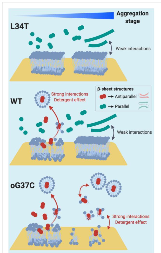
FIGURE 10 | Proposed Interaction schemes between A\beta_{1-42} L34T, WT, and oG37C peptide and POPC/SM/Chol/GM1 model membranes in early and late stages of amyloid aggregation. Anti-parallel \beta sheet structures are figured in red, while parallel \beta sheet structures are figured in green. Based on our observations in HS-AFM and NanoIR spectroscopy, strong interactions between the amyloid peptides and the membrane are only observed in the early stages of fibrillation, i.e., with small oligomers, and coincide with the presence of anti-parallel \beta sheet structures. These anti-parallel \beta sheet structures, similar to the oG37C toxic oligomer, would induce the dissolution of the membrane through a detergent effect.
