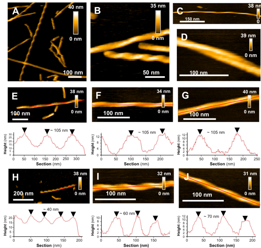
FIGURE 3 | L34T polymorphism and its evolution in time SHOWN BY HS-AFM images of L34T samples collected and observed after 7 (A,B) and 10 days fibrillation (C,D) showing several morphologies, with straight twisted fibers with short and long cross-over distances, curved fibers and mature filaments. (E–G) Evolution in time of periodic fibers with long and (H–J) shorter cross-over distance, acquired at days 1, 7 and 10, respectively. Height images are represented with a topographic cross section taken along the red line.
