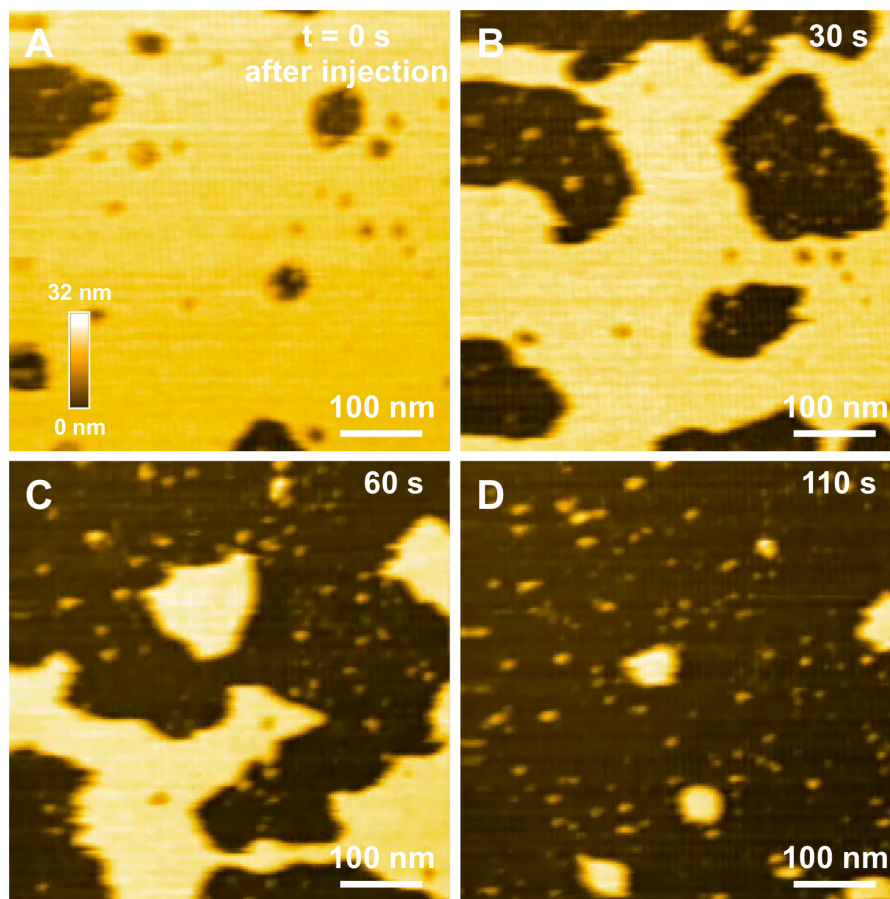
FIGURE 5 | Interaction between oG37C peptides and a POPC/SM/Chol/GM1 membrane. Successive HS-AFM height images extracted from video 2 at the time of injection ( A ), 30 s after injection ( B ), 60 s after injection ( C ), and 110 s after injection ( D ).
