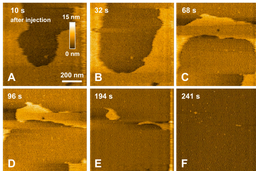
FIGURE 6 | Interaction between pre-fibrillar WT peptides and a POPC/SM/Chol/GM1 membrane. Successive HS-AFM height images extracted from video 3 10 s after injection (A), 32 s after injection (B), 68 s after injection (C), 96 s after injection (D), 194 s after injection (E), and 241 s after injection.
