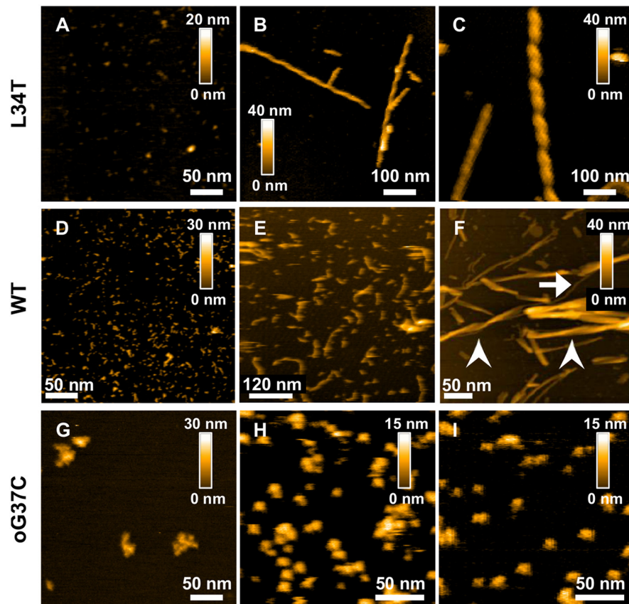
FIGURE 2 | Morphology of A \beta 1-42 WT and mutant peptides and their fibrillation products revealed by AFM height images obtained for L34T (A–C) WT (D–F), and oG37C (G–I) peptides at different times in the fibrillation process, with images acquired at day 0 (A,D,G), day 1 (B,H), day 2 (C,E,I), and day 7 (F). All peptides are incubated at 20 \mu l. White arrows indicates unique fibers, arrow-heads indicates fiber bundles.
