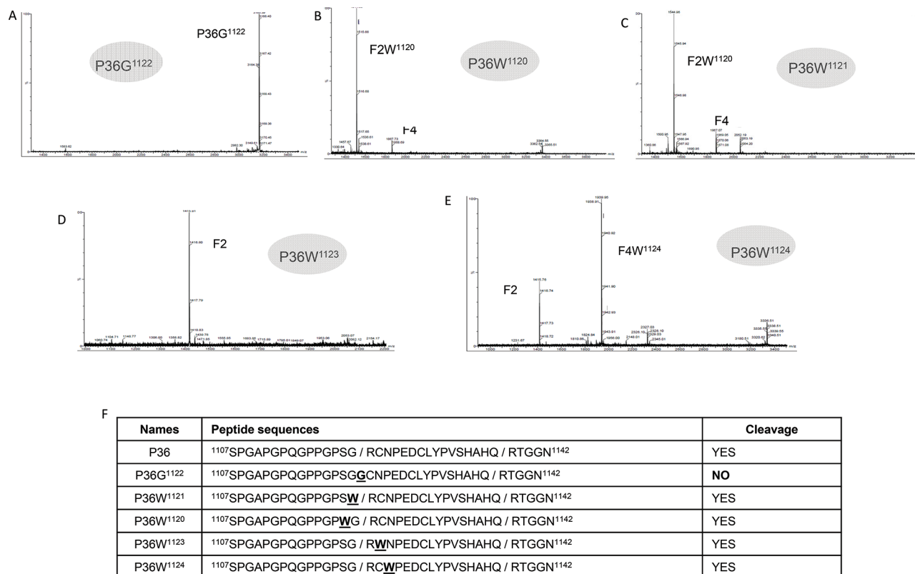
Figure 3: MALDI-ToF MS characterization of the substituted peptide after incubation with plasmin. (A) MALDI-ToF MS characterization of the substituted R 1122 to G 1122 P36 peptide after incubation with plasmin (E:S 1:50, 37°C overnight). No cleavage was observed. (B) MALDI-ToF MS characterization of the substituted S 1120 to W 1120 P36 peptide after incubation with plasmin (E:S 1:50, 37°C overnight). Complete digestion was observed. (C) MALDI-ToF MS characterization of the substituted G 1121 to W 1121 P36 peptide after incubation with plasmin (E:S 1:50, 37°C overnight). Complete digestion was observed. (D) MALDI-ToF MS characterization of the substituted C 1123 to W 1123 P36 peptide after incubation with plasmin (E:S 1:50, 37°C overnight). Complete digestion was observed. (E) MALDI-ToF MS characterization of the substituted N 1124 to W 1124 P36 peptide after incubation with plasmin (E:S 1:50, 37°C overnight). Complete digestion was observed. (F) Panel summarizing the cleavage of modified peptides by plasmin.
