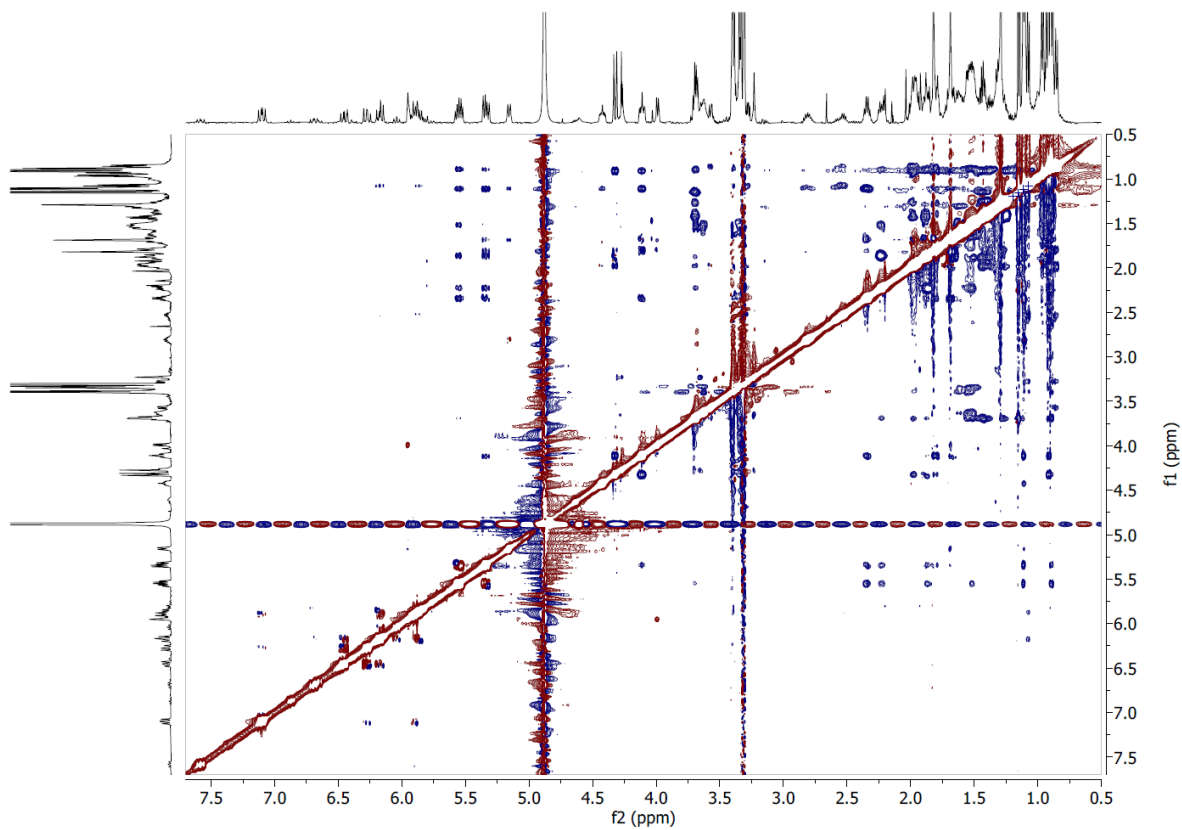
Figure S8: ROESY NMR spectrum of hemicialide in CD 3 OD
