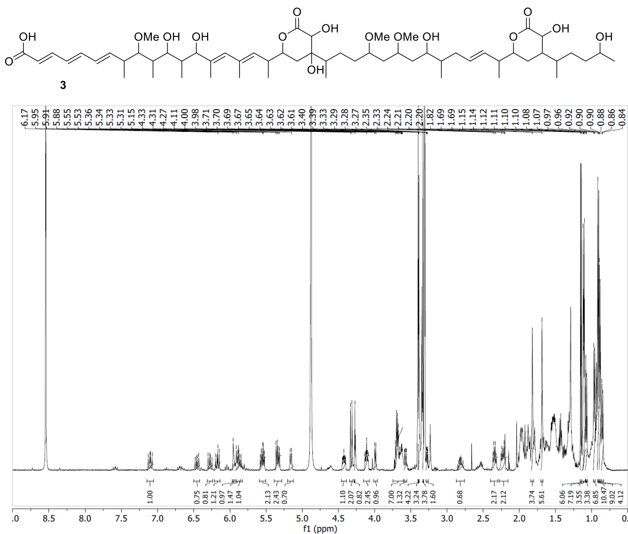
Figure S2: ^1\text{H} NMR spectrum of hemicalide in \text{CD}_3\text{OD} at 500 MHz
