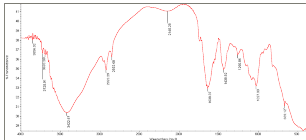
Figure 5. FTIR spectra of ALG–AG complex.
